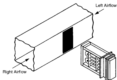
Figure 86B. Optional Slip-in Heater Installation
